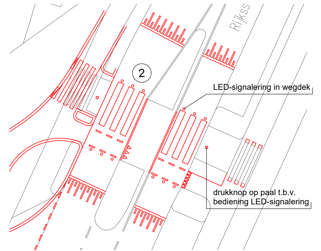
Detail LED-signalering VOP-FOP schaal 1:100
