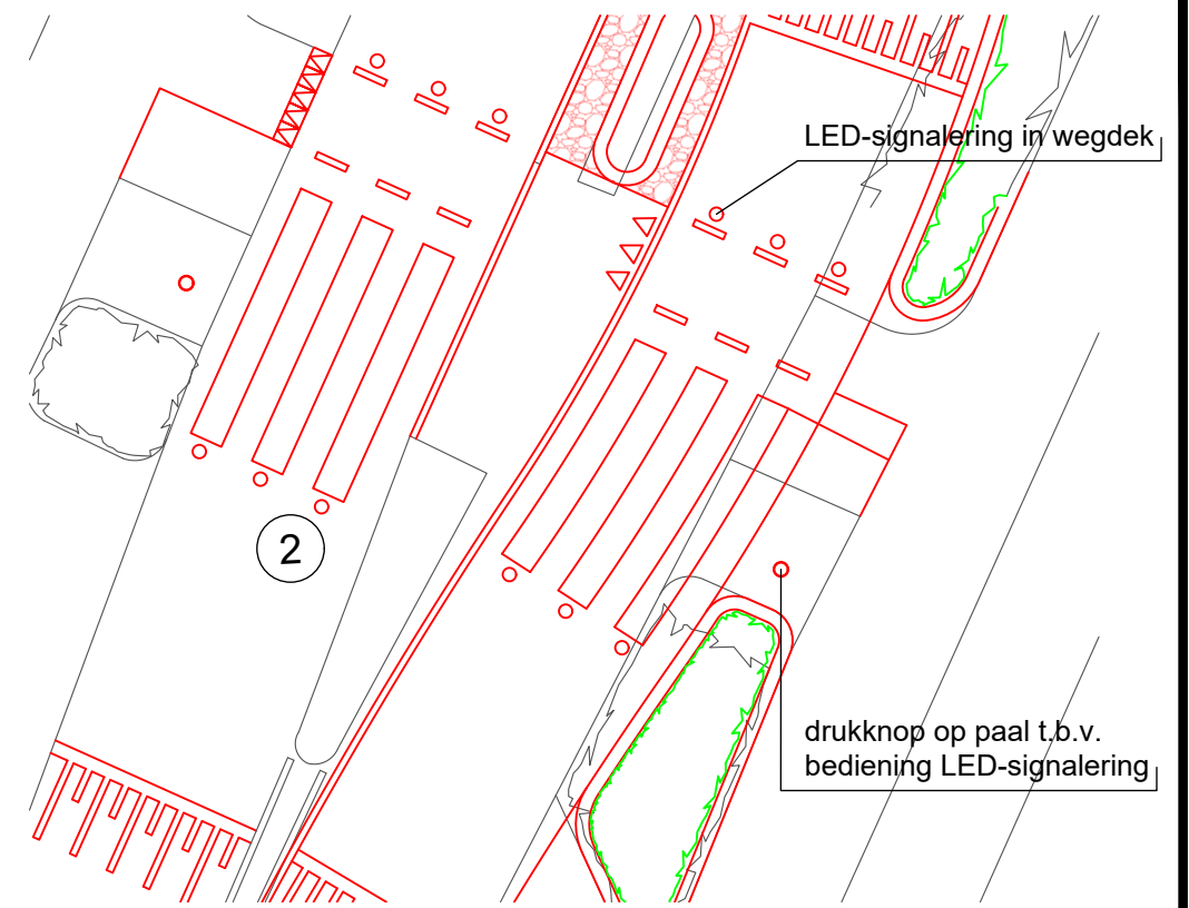
Detail LED-signaling VOP-FOP schaal 1:100
